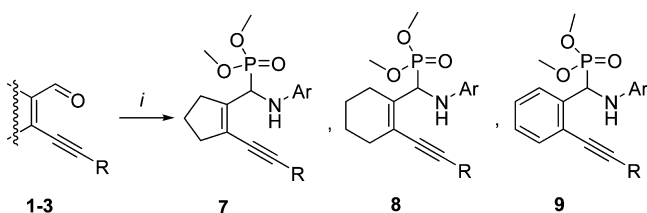
Scheme 2. Kabachnik–Fields Reaction of Carbocyclic Acetylenic Aldehydes 1–3 a
