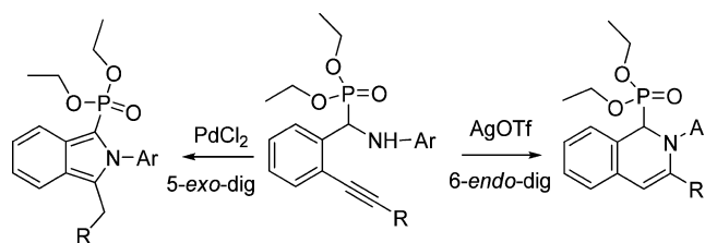
Scheme 1. Results of Ding et al. Published in 2007 5a
