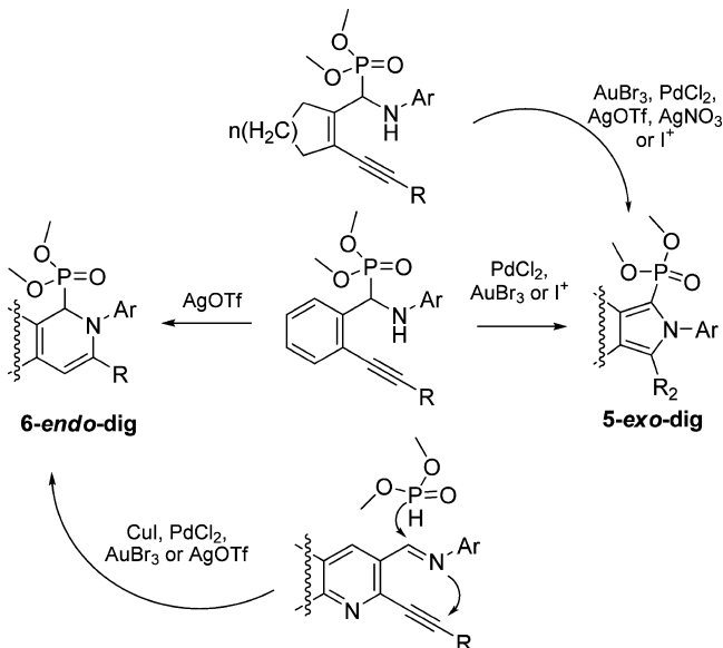
Scheme 7. Dependence of the Cyclization Mode on the Structures of the Starting Acetylenic \alpha -Anilinomethylphosphonates
