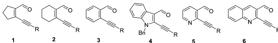
Figure 2. Starting acetylenic aldehydes. 1a: R = Ph; 1b: R = 4-MeC 6 H 4 ; 1c: R = 4-EtC 6 H 4 ; 1d: R = Bu; 1e: R = C 5 H 11 ; 1f: R = c -Pr; 1g: R = TMS. 2a: R = Ph; 2b: R = 4-MeC 6 H 4 ; 2c: R = Pr; 2d: R = Bu; 2e: R = C 5 H 11 ; 2f: R = c -Pr. 3a: R = Ph; 3b: R = TMS. 4a: R = Ph; 4b: R = Bu; 4c: R = c -Pr. 5a: R = Ph; 5b: R = Pr; 5c: R = c -Pr; 5d: R = H; 5e: R = CH 2 OTHP. 6a: R = Ph; 6b: R = Bu; 6c: R = Pr; 6d: c -Pr.
