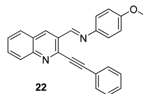
Figure 3. ( E )-4-Methoxy- N -{[2-(phenylethynyl)quinolin-3-yl]-methylene}aniline 22 .
