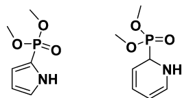
Figure 1. Structures of 1 H -pyrrol-2-ylphosphonate and 1,2-dihydropyridin-2-ylphosphonate.
